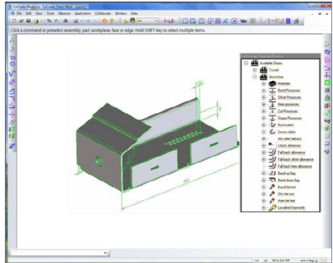
The Sheet Metal knowledge database with the manufacturing tools ensure the manufacturability of the design
