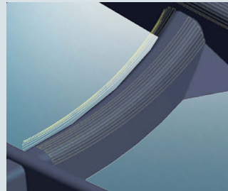
3D ISO Finishing of fillets
