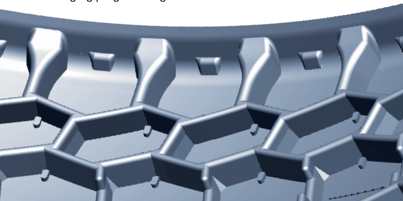
5axis Swarf machining with conical ball mill
