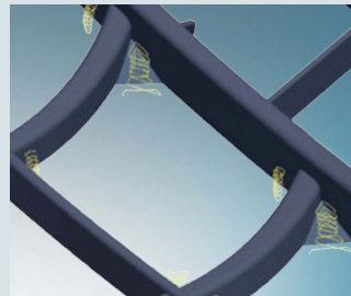
5axis Shape Finishing in rest machining mode
