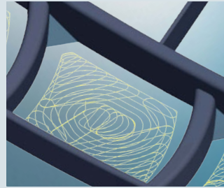
5axis Shape Roughing with hyperMAXX ®: 5axis trochoidal-style machining
